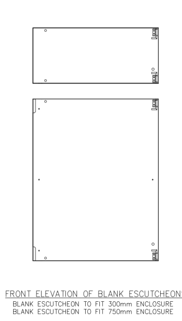
FRONT ELEVATION MOUNTING RAILS FITTED SEGREGATION TOP AND BOTTOM PIECES FITTED SEGREGATION TO MATCH 300M/750MM ESCUTCHEON HEIGHTS
