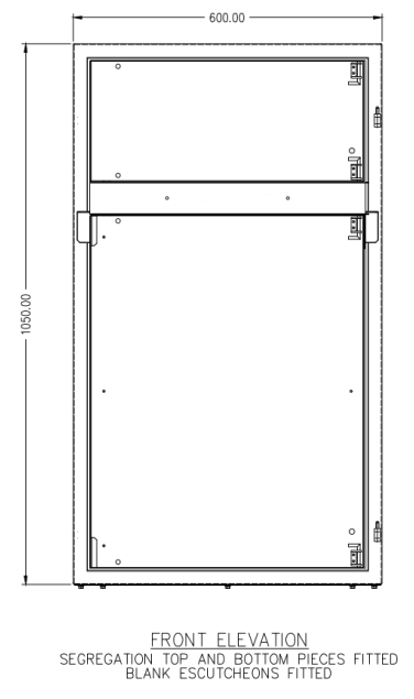
FRONT ELEVATION OF BLANK ESCUTCHEONS BLANK ESCUTCHEON TO FIT 300mm ENCLOSURE BLANK ESCUTCHEON TO FIT 750mm ENCLOSURE
